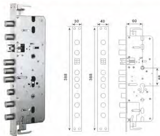
National standard 6068 stainless steel lock body (large overlord)
