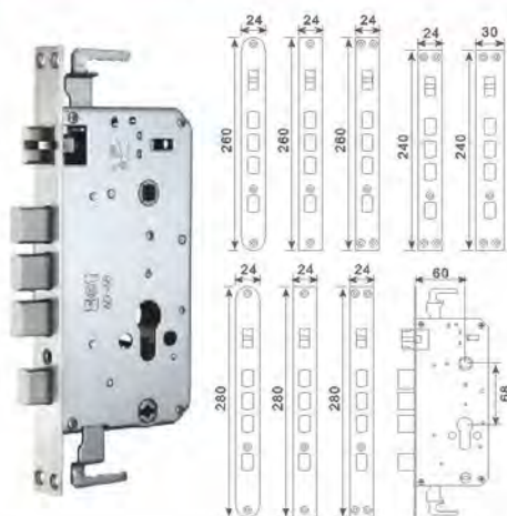
National standard 6068 stainless steel lock body (large overlord)
