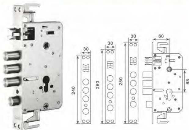
Gb 6068 stainless steel cylinder lock body (medium)
